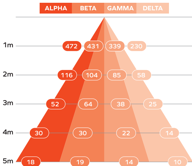
HALO 3 - 24VDC LIGHT GRAPH
