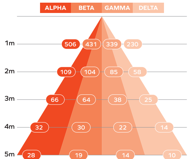
HALO 3 - 48VDC LIGHT GRAPH
